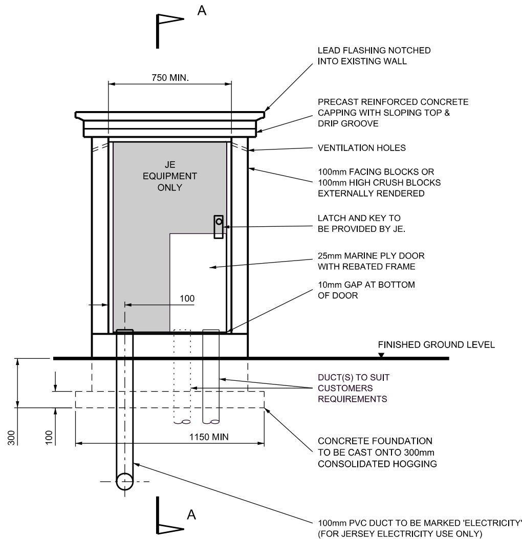
FRONT ELEVATION
