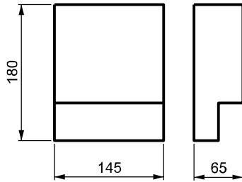
Liberty 140 single phase meters. (General tariff)
